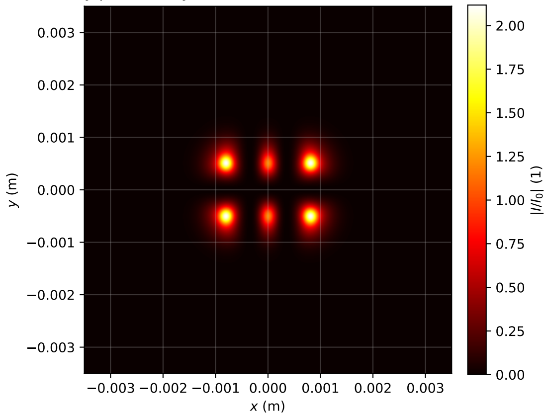
Intensity profile I(x, y, z = 0.318)/I_0 , P_{in}=7.0P_{cr} , artificial time
